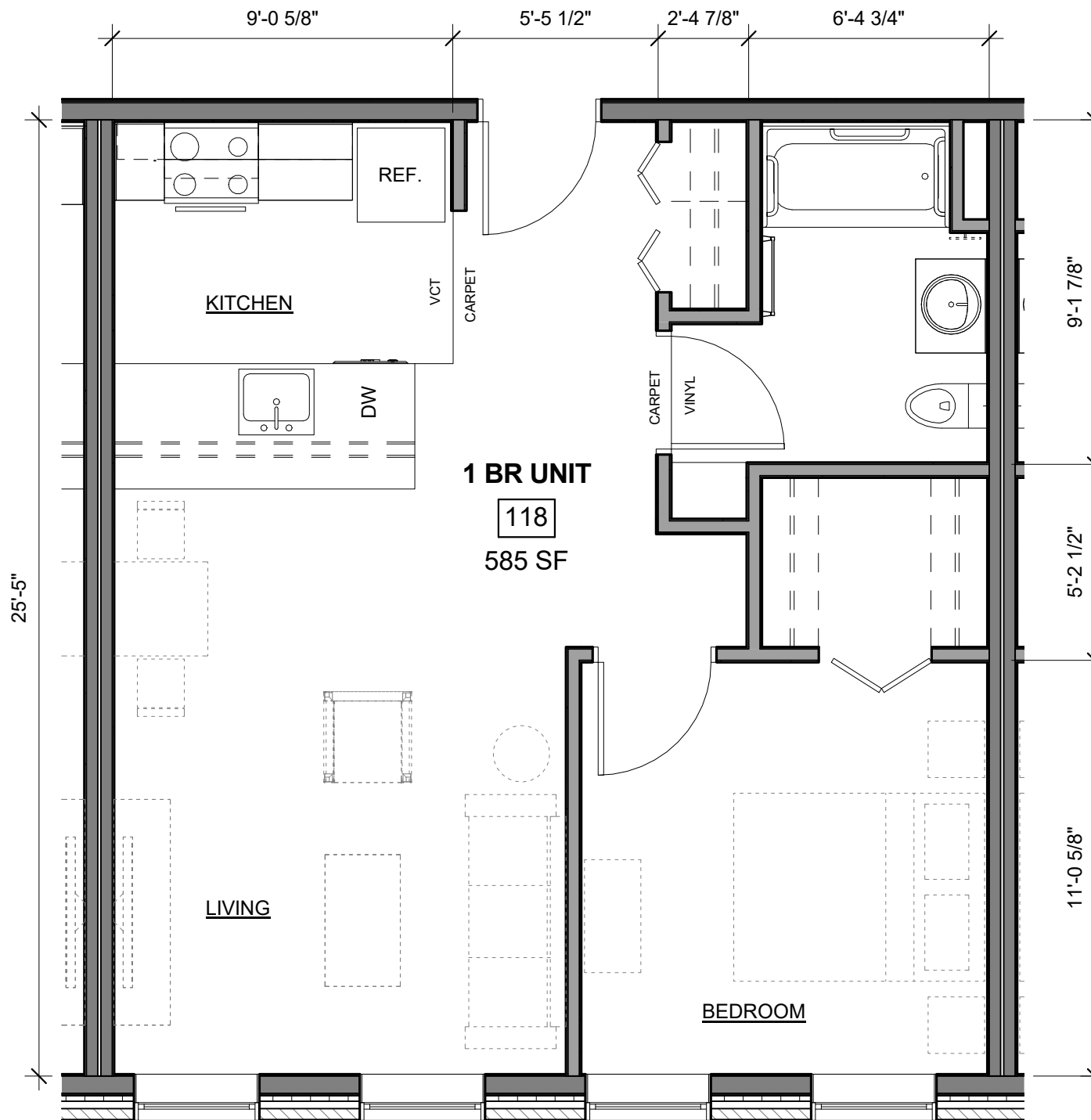
1 | ENLARGED UNIT PLAN - 1 BEDROOM 1/4" = 1'-0"
