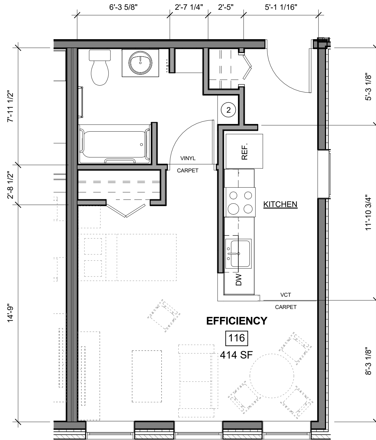
1 | ENLARGED UNIT PLAN - EFFICIENCY 1/4" = 1'-0"
