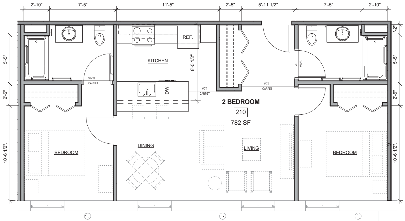
1 | ENLARGED UNIT PLAN - 2 BEDROOM 1/4" = 1'-0"
