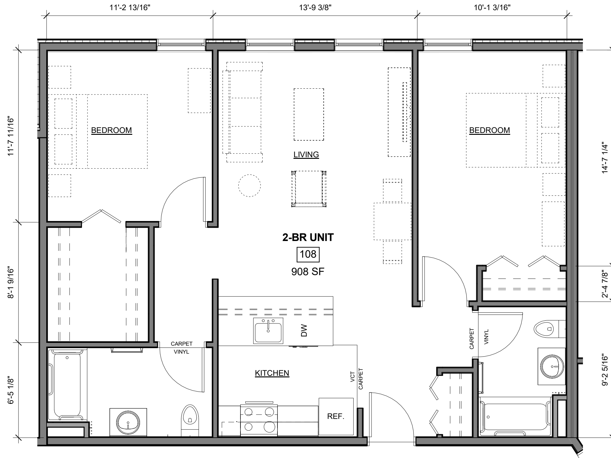
1 | ENLARGED UNIT PLAN - 2 BEDROOM 1/4" = 1'-0"
