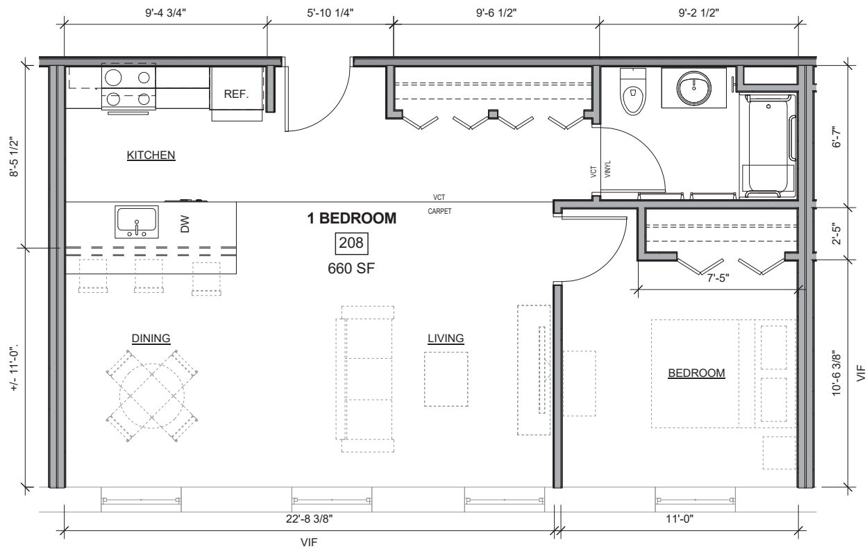
1 | ENLARGED UNIT PLAN - 1 BEDROOM 1/4" = 1'-0"
